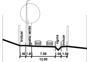
PROFIL TRANSVERSAL PROPUȘ DRUM CAROSABIL sc. 1/500
